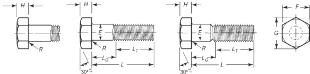
Bolt With Reduced Diameter Body
